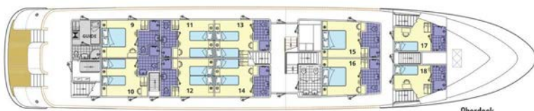
Oberdeck
